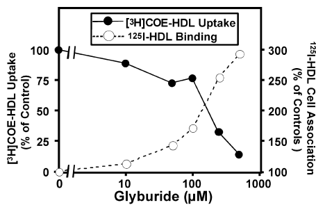
Fig. 5. Effects of glyburide on SR-BI-mediated [ 3 H]cholesteryl oleyl ether ([ 3 H]COE) uptake from [ 3 H]COE-HDL and 125 I-HDL binding. SR-BI-expressing ldlA[mSR-BI] or control ldlA-7 cells were preincubated with the indicated concentrations of glyburide, and then the uptake of [ 3 H]COE from [ 3 H]COE-HDL (10 µg protein/ml) (closed circles) or the binding of 125 I-HDL (10 µg protein/ml) (open circles) was determined in the presence or absence of a 40-fold excess of unlabeled HDL (duplicate incubations). The specific values (difference between the values in the absence and presence of excess HDL) were normalized such that the value in the absence of glyburide was set to 100%. The 100% of control values (nanograms of HDL protein per milligram of cell protein) for ldlA[mSR-BI] cells were as follows: [ 3 H]COE uptake, 1,962; 125 I-HDL binding, 198. The 100% of control values for ldlA-7 cells were as follows: [ 3 H]COE uptake, 289; 125 I-HDL binding, 21.
