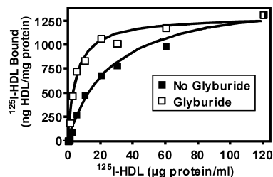
Fig. 6. Effects of glyburide on the concentration dependence of 125 I-HDL binding to SR-BI-expressing cells. SR-BI-expressing ldlA[mSR-BI] cells were preincubated in the absence (closed squares) or presence (open squares) of 250 µM glyburide and then incubated for 2 h at 37°C with the same amount of glyburide and the indicated concentrations of 125 I-HDL in the presence (single incubations) or absence (duplicate incubations) of a 40-fold excess of unlabeled HDL. The specific binding values are shown.
