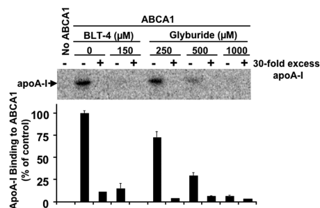
Fig. 7. Effects of BLT-4 and glyburide on 125 I-apoA-I binding to ABCA1. HEK293-EBNA-T cells were transiently transfected with either an ABCA1 expression vector (ABCA1) or a control pcDNA1 vector (No ABCA1). One day after transfection, the cells were preincubated for 1 h at 37°C in assay medium with the indicated concentrations of BLT-4 or glyburide. The binding of 125 I-apoA-I (2 µg/ml, 1 h, 37°C) in the presence or absence of a 30-fold excess of unlabeled apoA-I and the indicated concentrations of inhibitors was measured using a dithiobis (succinimidyl propionate) cross-linking assay as described in Experimental Methods. Bound 125 I-apoA-I was fractionated by SDS-PAGE and detected in the gels using a PhosphorImaging STORM860 system (top), and the relative amounts of 125 I-apoA-I in the lanes were determined using ImageQuant software (bottom). Values shown in the lower portion of the figure are representative of two independent experiments performed in duplicate. Error bars represent the ranges of duplicate determinations.
