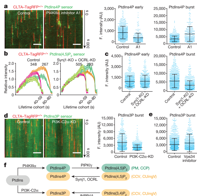
Figure 3 | Interference of phosphoinositide kinases and phosphatases on phosphoinositide content of endocytic clathrin-coated structures. a, Inhibition of PI4KIIIα lowered accumulation of PtdIns4P sensor during coated pit assembly. CLTA-TagRFP +/+ cells stably expressing the PtdIns4P sensor EGFP-P4M(DrrA)-Aux1 were treated with dimethyl sulfoxide (DMSO; control) or the PI4KIIIα inhibitor A1. Representative kymographs and sensor intensities from 738 and 303 traces from 5 control and 14 treated cells, respectively. A1 significantly decreased early PtdIns4P content (Cohen's d = 0.89 ) and increased burst amplitude (Cohen's d = 1.06 ). b, Eliminating Synj1 and depleting OCRL by 80% increased recruitment of the PtdIns(4,5)P 2 sensor to clathrin-coated structures. The PtdIns(4,5)P 2 sensor EGFP-PH(PLCδ1)-Aux1 was transiently expressed in control or Synj1-knockout (KO) CLTA-TagRFP +/+ cells treated with control or OCRL siRNA (OCRL-KD). Plots show averaged fluorescence (F) intensity traces of clathrin and the PtdIns(4,5)P 2 sensor associated with endocytic coated pits, including the numbers of analysed traces from 10 control and 11 Synj1-KO + OCRL-KD cells. c, Synj1-KO + OCRL-KD diminished PtdIns4P sensor burst during uncoating (Cohen's d = 0.72 ) but had no effect on early PtdIns4P content of coated pits (Cohen's d = 0.04 ); 895 and 704 traces from 9 control and 11 Synj1-KO + OCRL-KD cells, respectively. d, PI3K-C2α knockdown in CLTA-TagRFP +/+ cells stably expressing PtdIns3P sensor EGFP-2×FYVE(Hrs)-Aux1 significantly decreased the late burst of sensor (Cohen's d = 0.81 ); 769 and 1,004 traces from 11 control and 13 PI3K-C2α-KD cells, respectively. e, Inhibition of Vps34 by PIK-III in CLTA-TagRFP +/+ cells expressing the PtdIns3P sensor EGFP-2×FYVE(Hrs)-Aux1 had a minor effect on sensor burst (Cohen's d = 0.21 ); 1,695 and 742 traces from 7 control and 7 treated cells, respectively. f, Phosphoinositide kinases and phosphatases responsible for phosphoinositide interconversion in clathrin-mediated endocytic traffic. CCP, clathrin-coated pit; CCV, clathrin-coated vesicle; CUingV, clathrin-coated vesicle undergoing uncoating; PM, plasma membrane. Data from TIRF microscopy (300 s, 1-s intervals); EGFP signal in the kymographs laterally shifted six pixels. Scale bars, 5 μm. See Methods for statistics.
